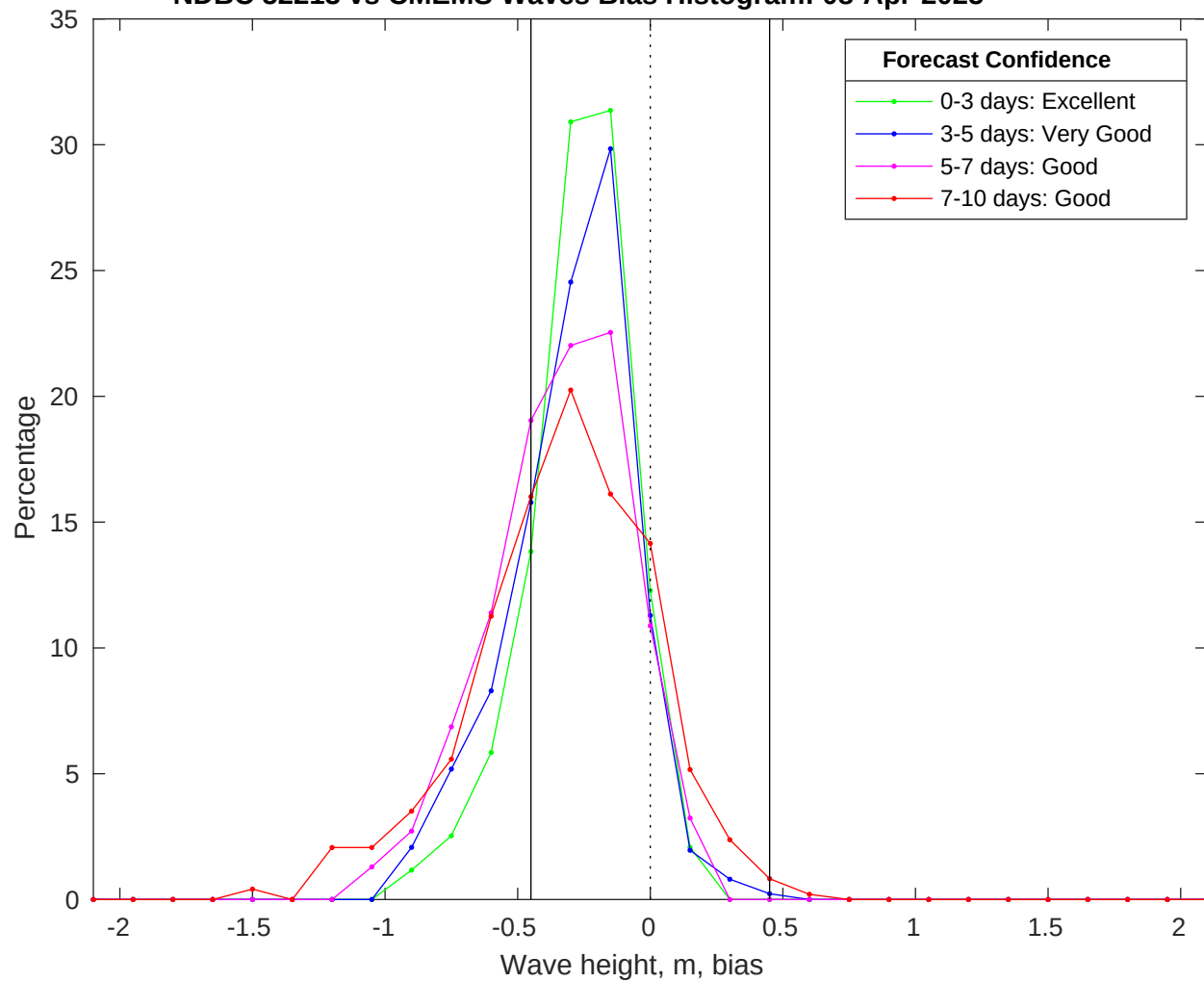
NDBC 52213 vs CMEMS Waves Bias Histogram: 08-Apr-2025
