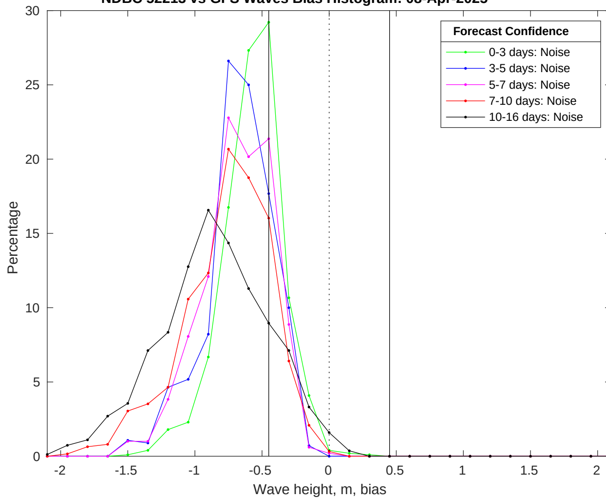
NDBC 52213 vs GFS Waves Bias Histogram: 08-Apr-2025
