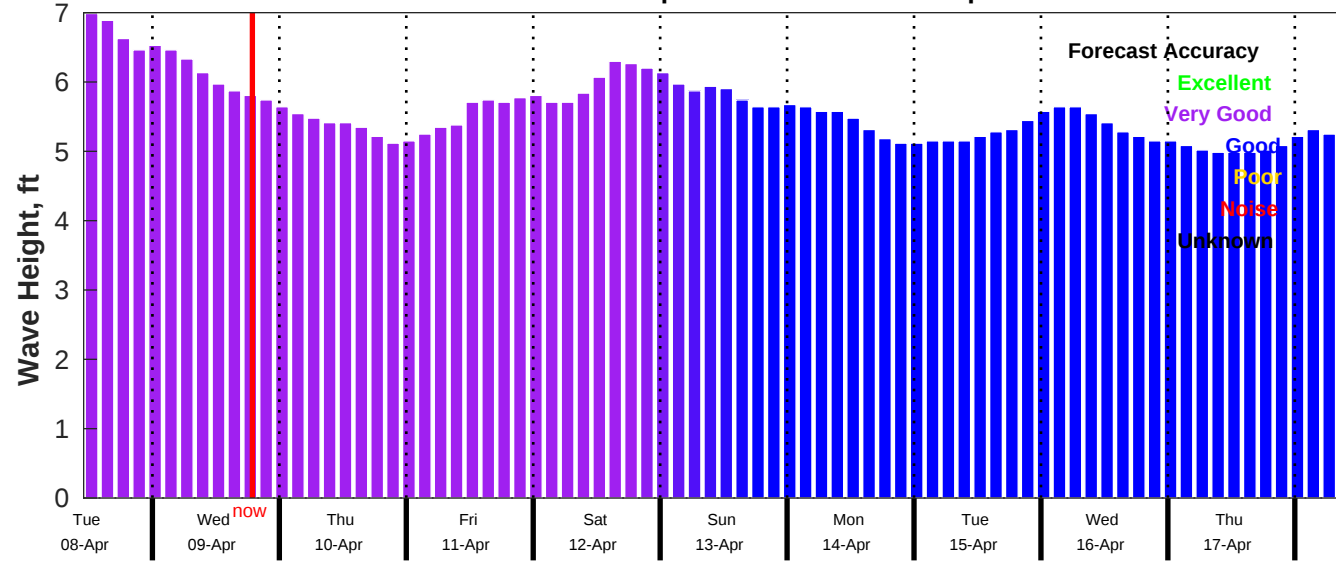
CMEMS Wave Forecast for NDBC 52213 from 07-Apr-2025 11:00:00 to 17-Apr-2025 11:00:00
