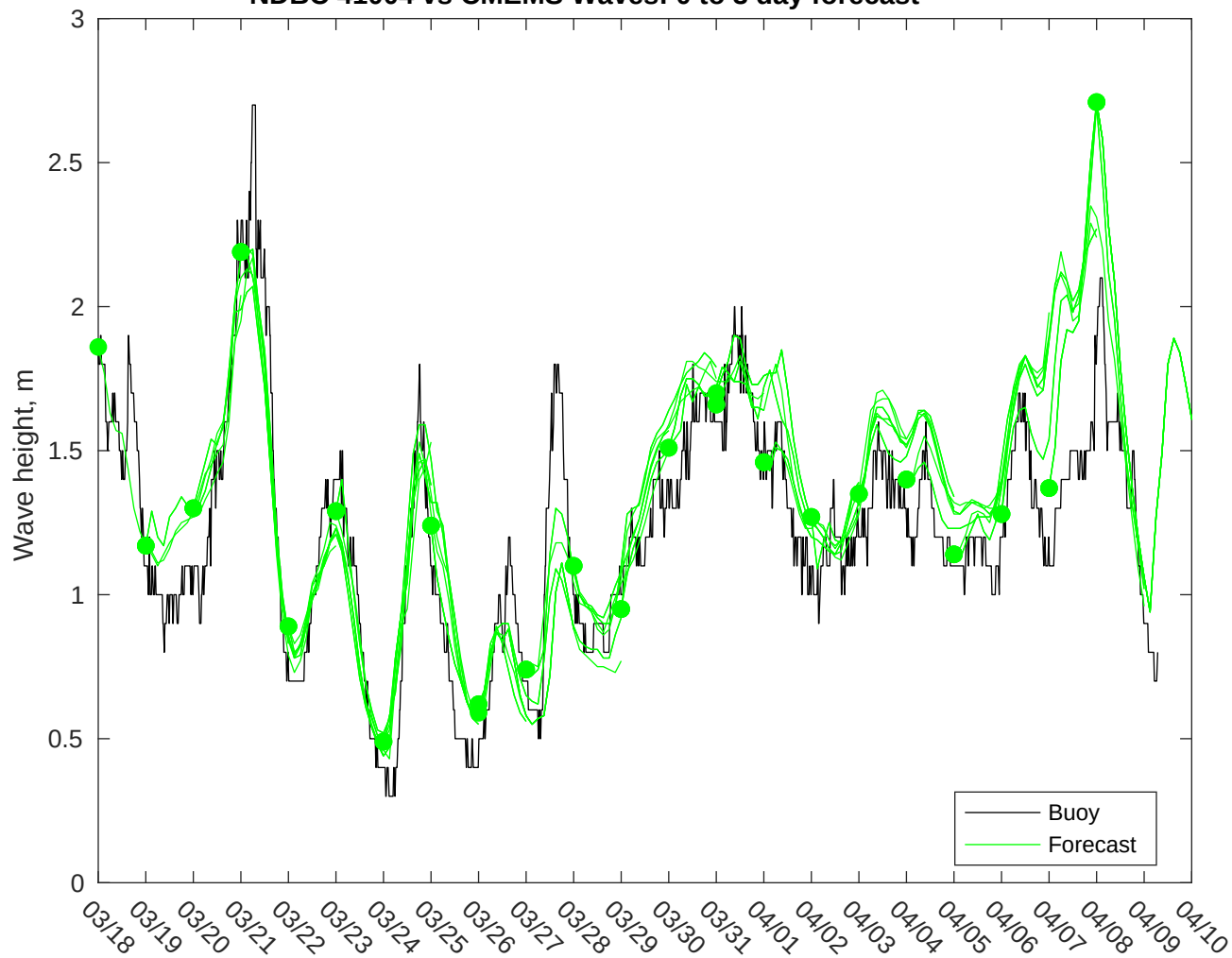
NDBC 41004 vs CMEMS Waves: 0 to 3 day forecast
