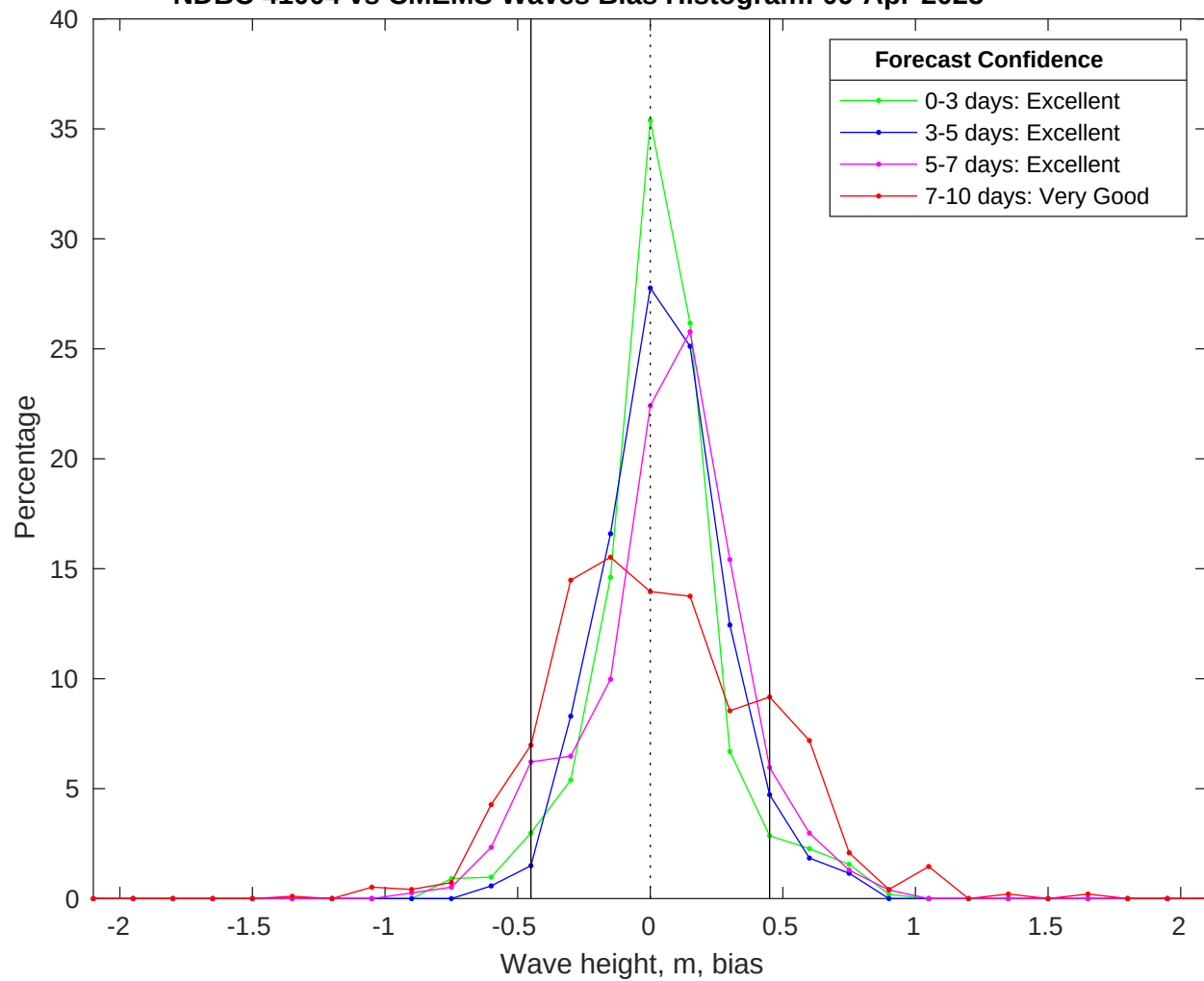
NDBC 41004 vs CMEMS Waves Bias Histogram: 09-Apr-2025
