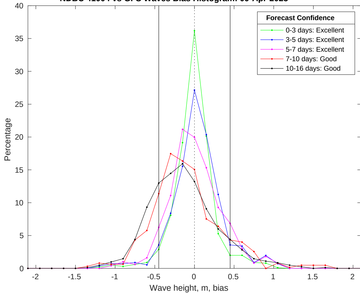
NDBC 41004 vs GFS Waves Bias Histogram: 09-Apr-2025
