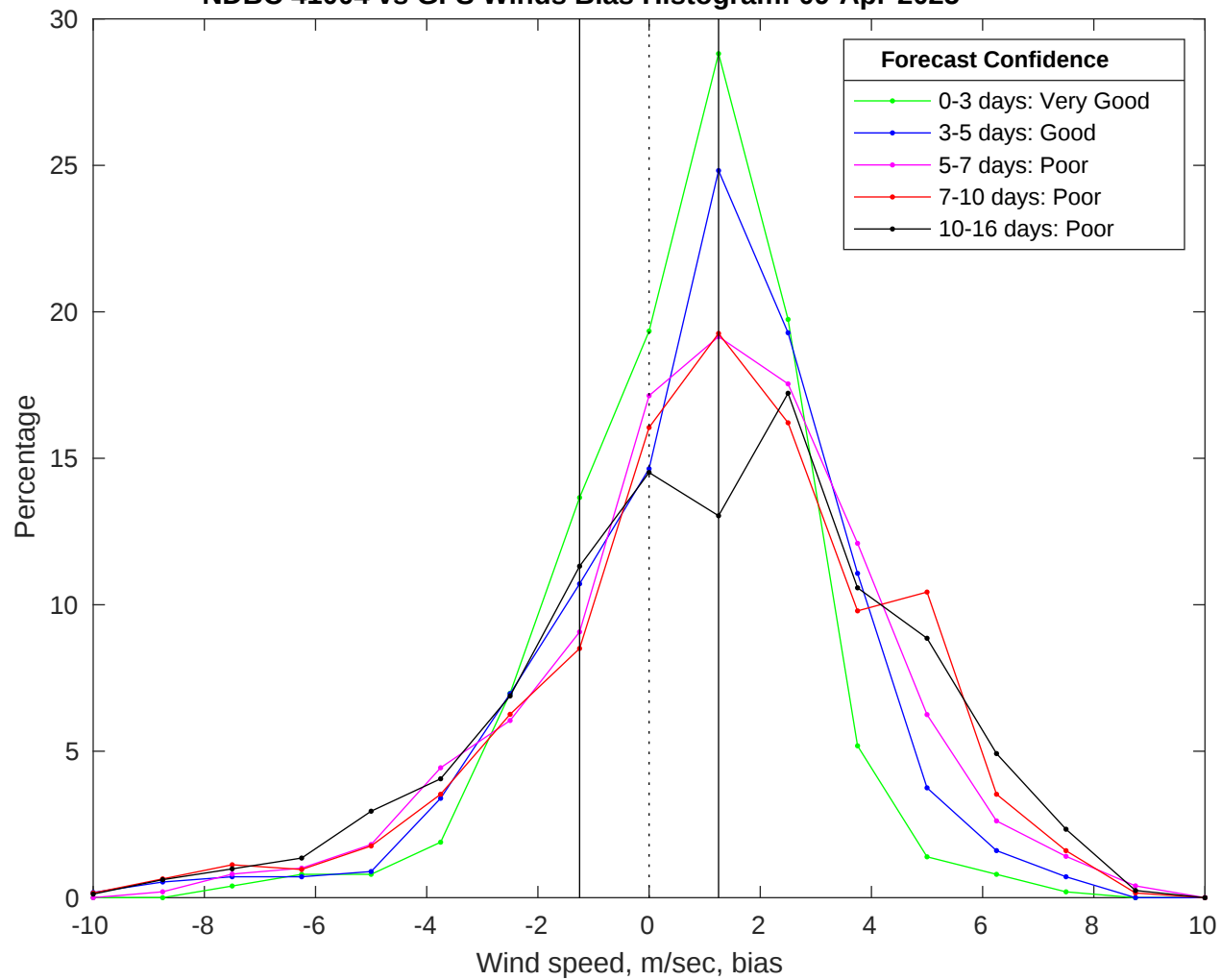
NDBC 41004 vs GFS Winds Bias Histogram: 09-Apr-2025
