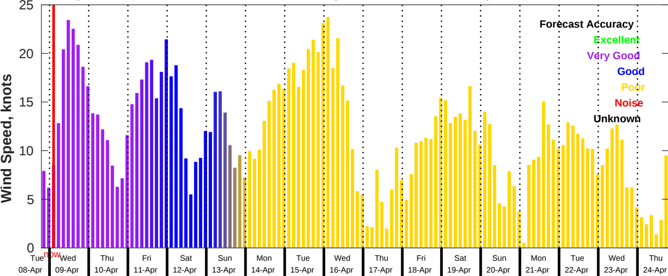
GFS Wind Speed Forecast for NDBC 41004 from 08-Apr-2025 19:00:00 to 24-Apr-2025 19:00:00
