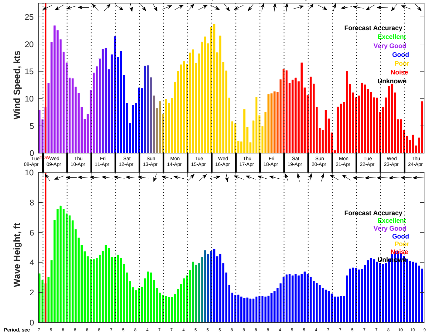
Wind & Wave Forecast for NDBC 41004 from 08-Apr-2025 19:00:00 to 24-Apr-2025 19:00:00
