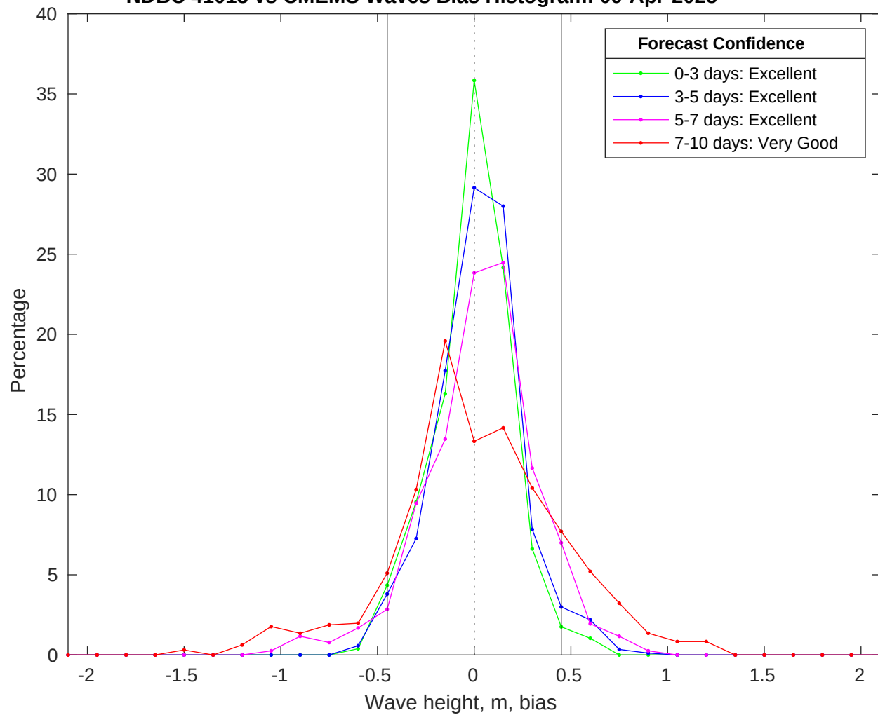
NDBC 41013 vs CMEMS Waves Bias Histogram: 09-Apr-2025
