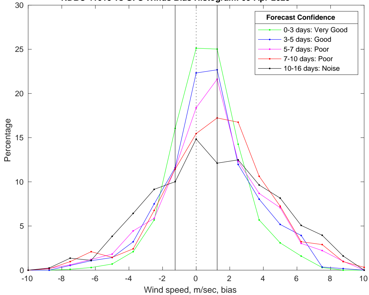
NDBC 41013 vs GFS Winds Bias Histogram: 09-Apr-2025
