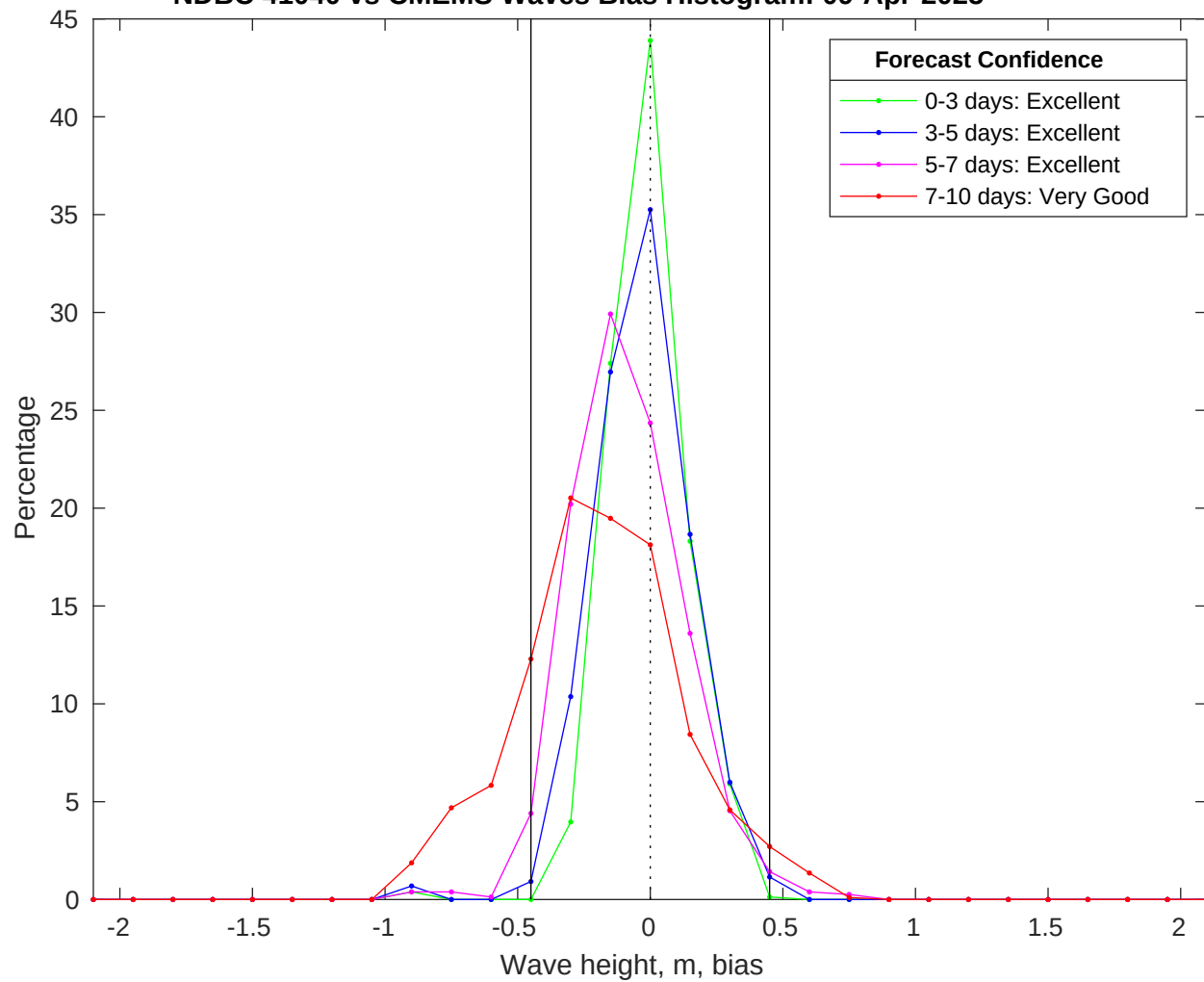
NDBC 41040 vs CMEMS Waves Bias Histogram: 09-Apr-2025
