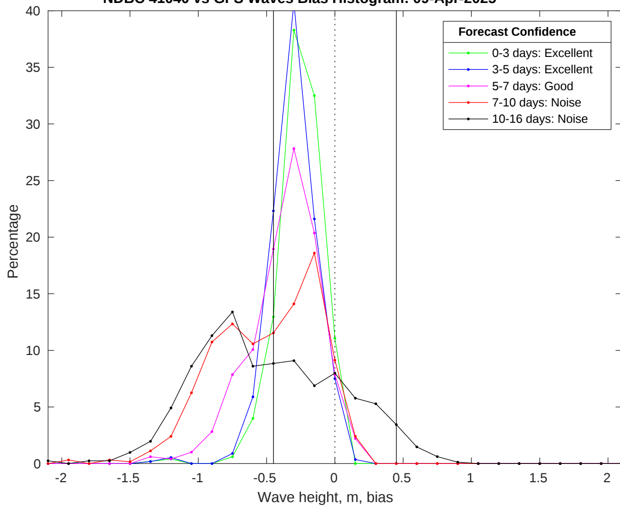
NDBC 41040 vs GFS Waves Bias Histogram: 09-Apr-2025
