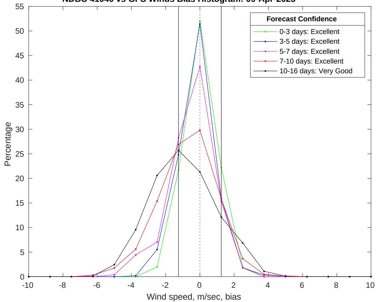
NDBC 41040 vs GFS Winds Bias Histogram: 09-Apr-2025
