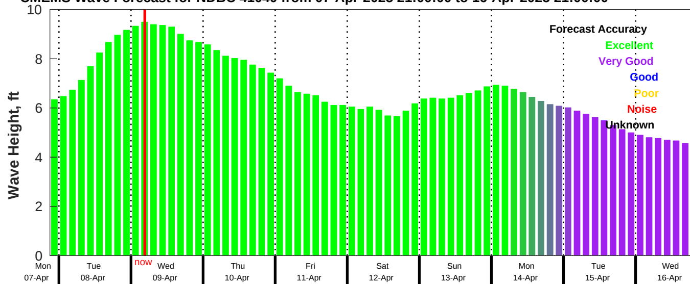
CMEMS Wave Forecast for NDBC 41040 from 07-Apr-2025 21:00:00 to 16-Apr-2025 21:00:00
