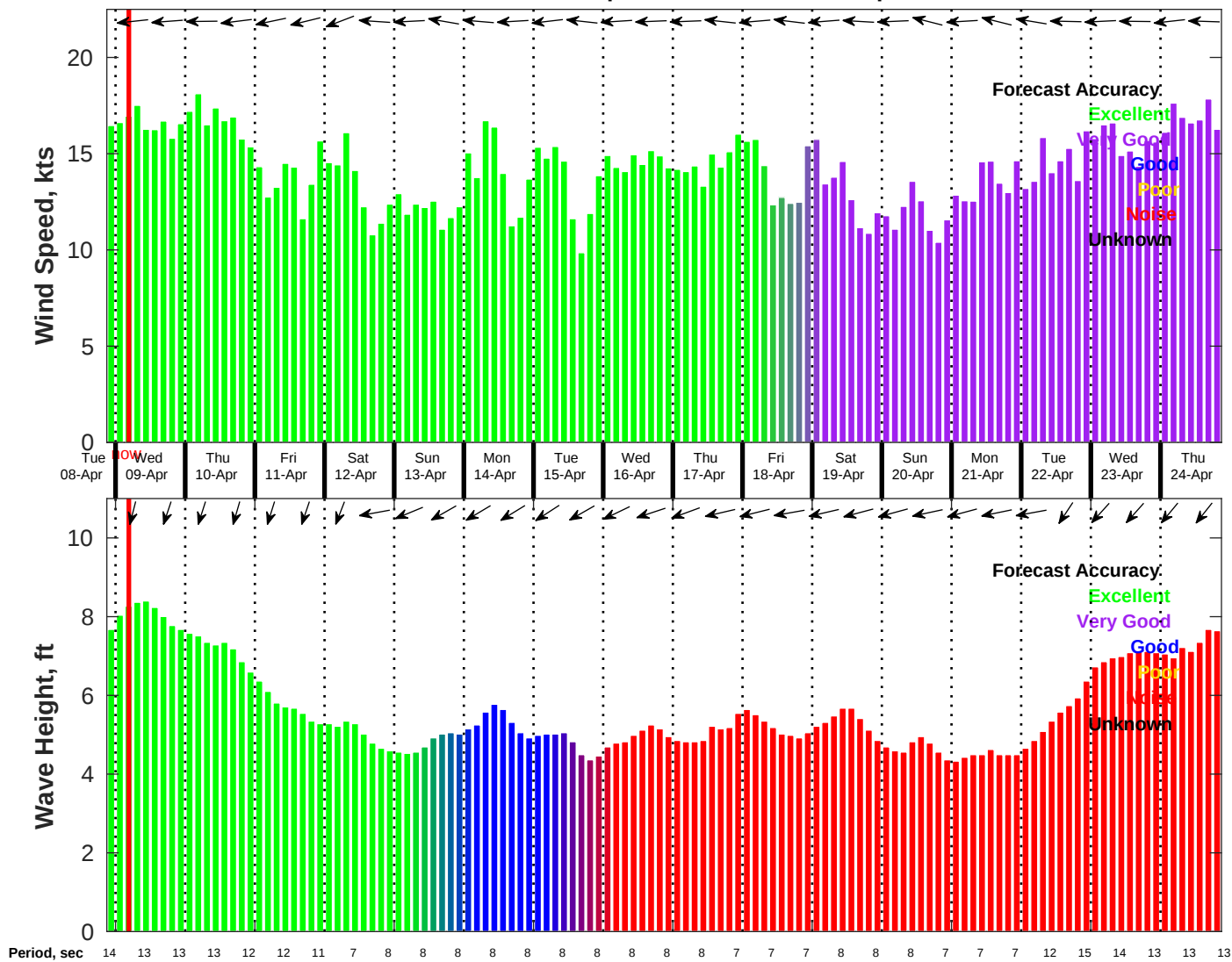
Wind & Wave Forecast for NDBC 41040 from 08-Apr-2025 21:00:00 to 24-Apr-2025 21:00:00
