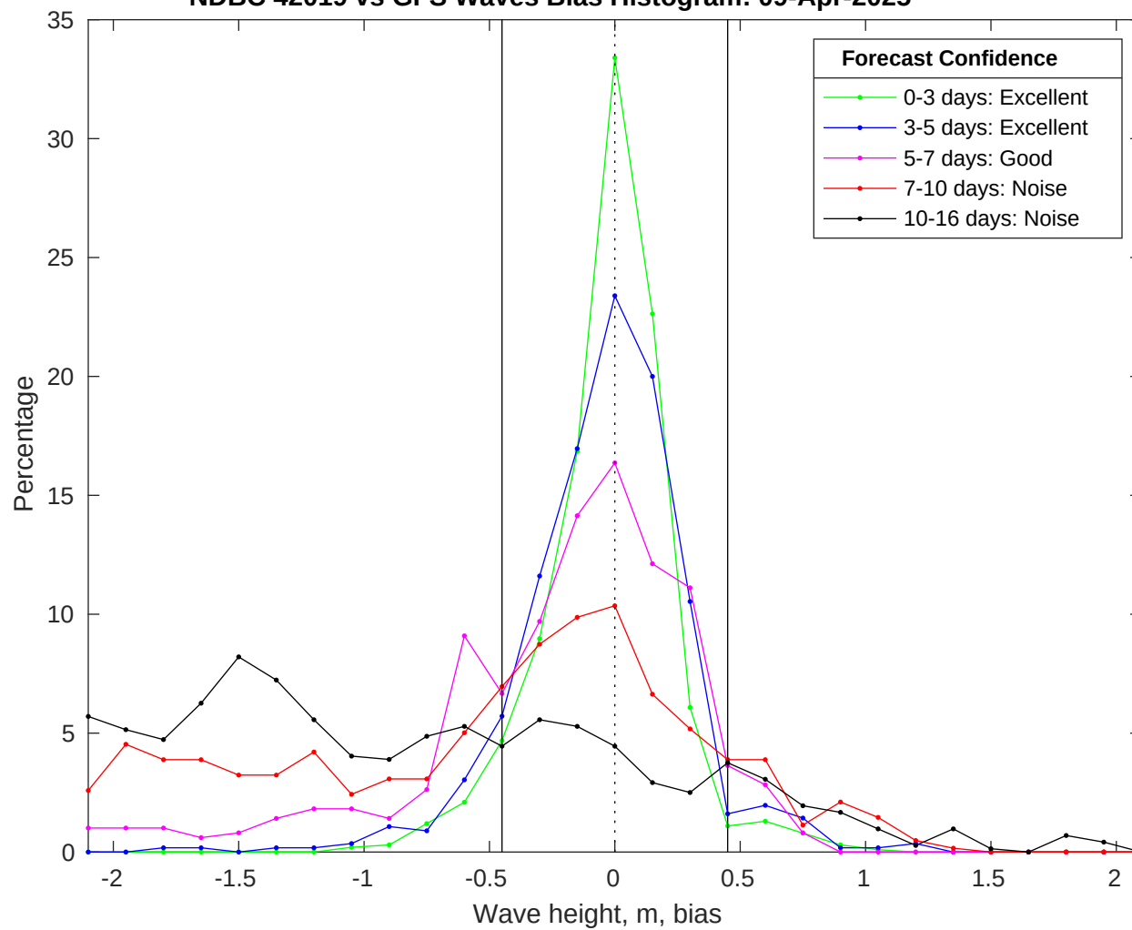
NDBC 42019 vs GFS Waves Bias Histogram: 09-Apr-2025
