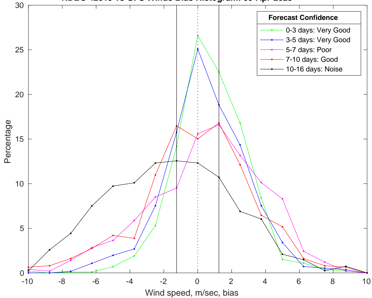
NDBC 42019 vs GFS Winds Bias Histogram: 09-Apr-2025
