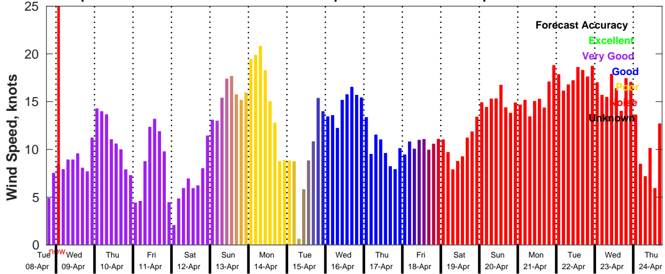
GFS Wind Speed Forecast for NDBC 42019 from 08-Apr-2025 18:00:00 to 24-Apr-2025 18:00:00
