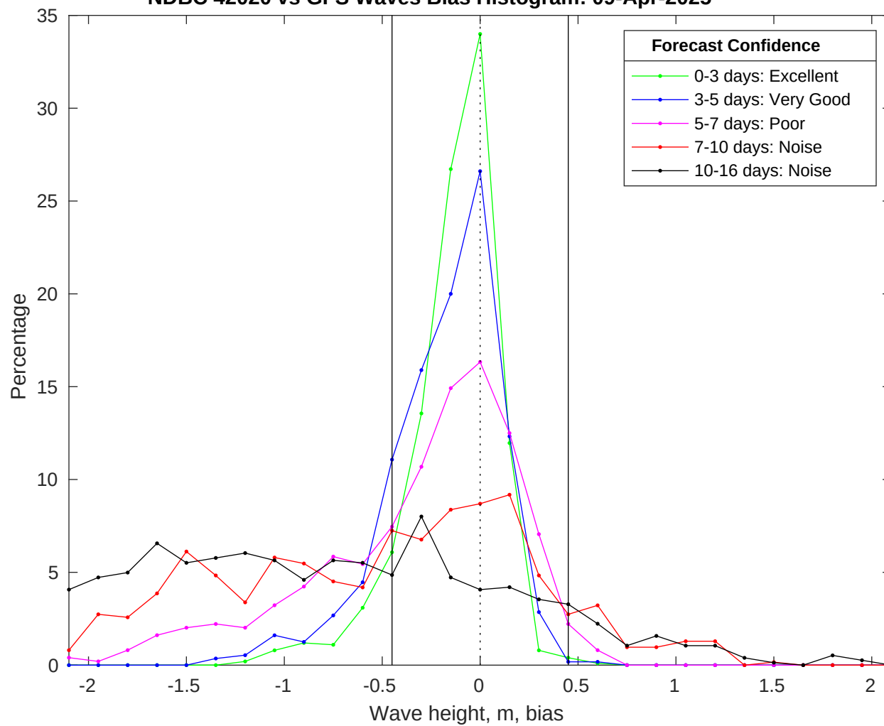
NDBC 42020 vs GFS Waves Bias Histogram: 09-Apr-2025
