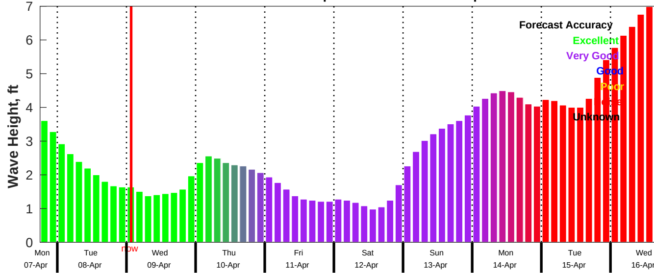
CMEMS Wave Forecast for NDBC 42020 from 07-Apr-2025 18:00:00 to 16-Apr-2025 18:00:00
