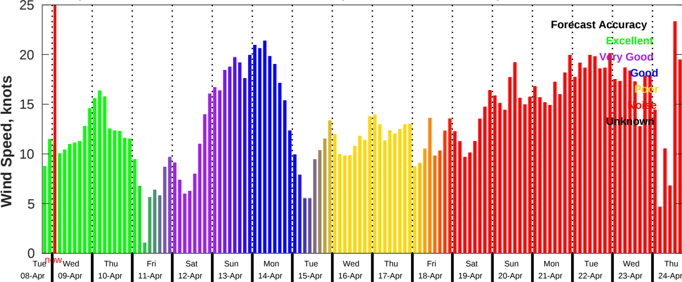
GFS Wind Speed Forecast for NDBC 42020 from 08-Apr-2025 18:00:00 to 24-Apr-2025 18:00:00
