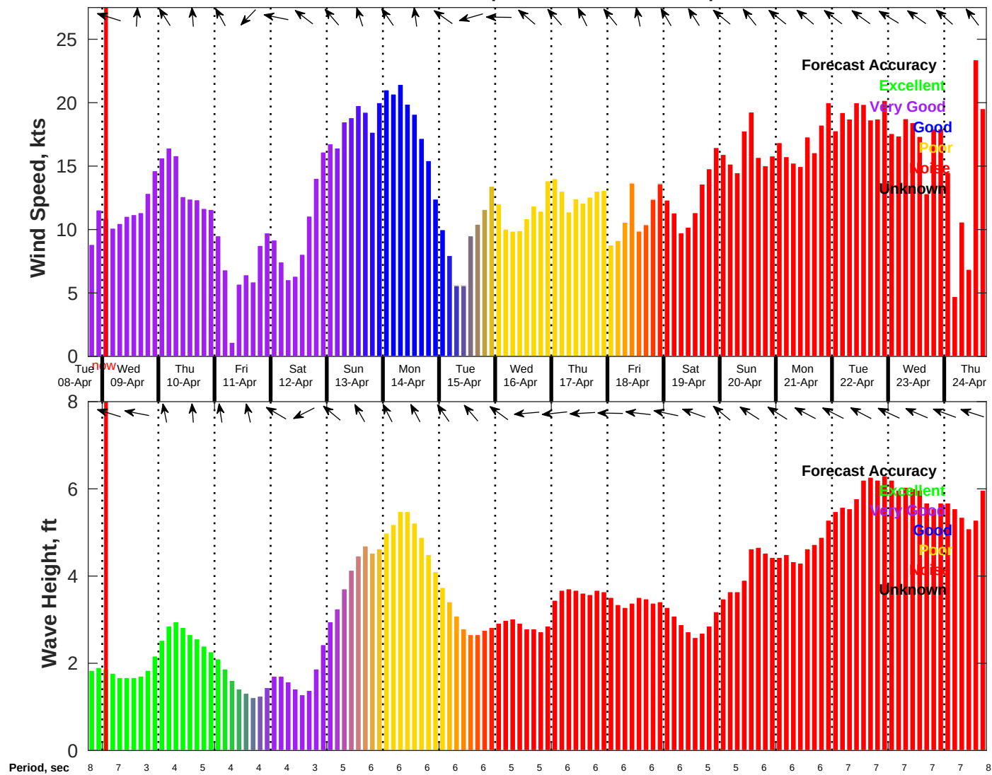
Wind & Wave Forecast for NDBC 42020 from 08-Apr-2025 18:00:00 to 24-Apr-2025 18:00:00
