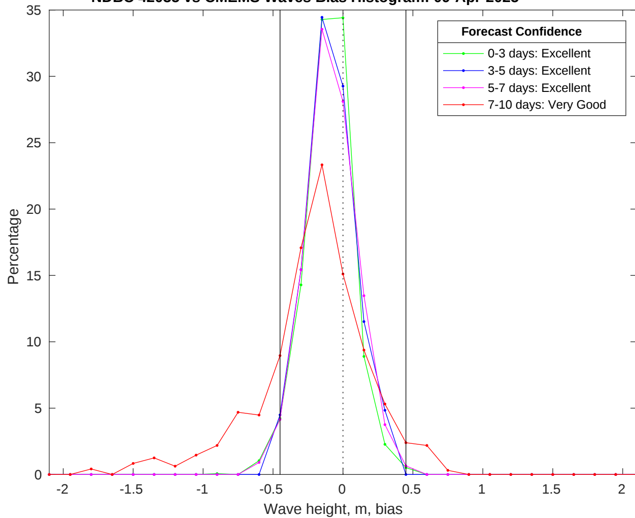
NDBC 42035 vs CMEMS Waves Bias Histogram: 09-Apr-2025
