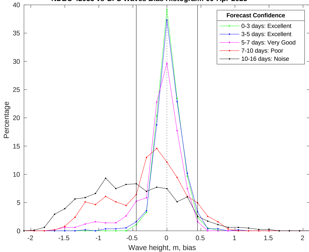
NDBC 42035 vs GFS Waves Bias Histogram: 09-Apr-2025
