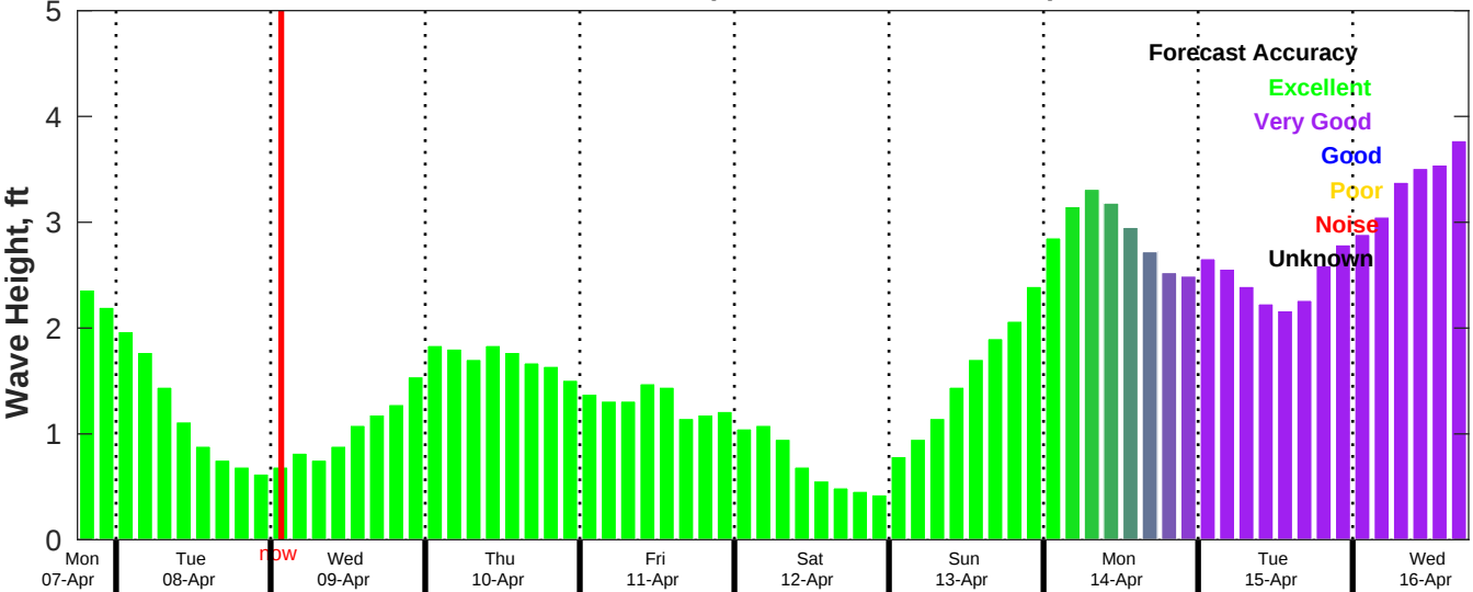
CMEMS Wave Forecast for NDBC 42035 from 07-Apr-2025 18:00:00 to 16-Apr-2025 18:00:00
