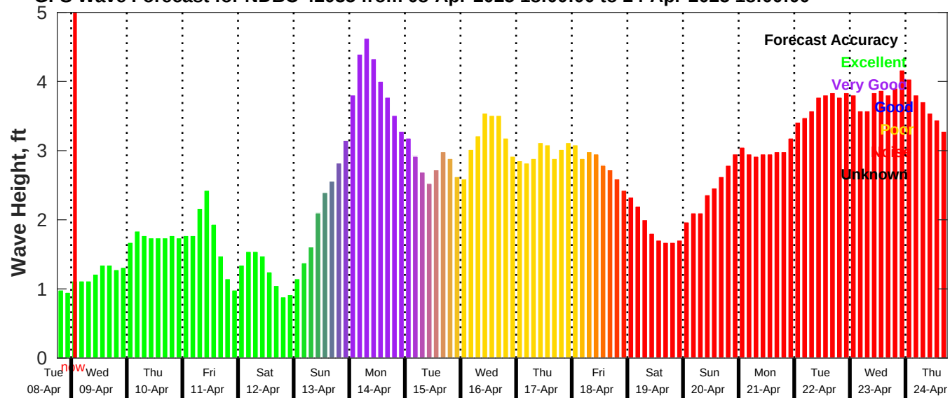
GFS Wave Forecast for NDBC 42035 from 08-Apr-2025 18:00:00 to 24-Apr-2025 18:00:00
