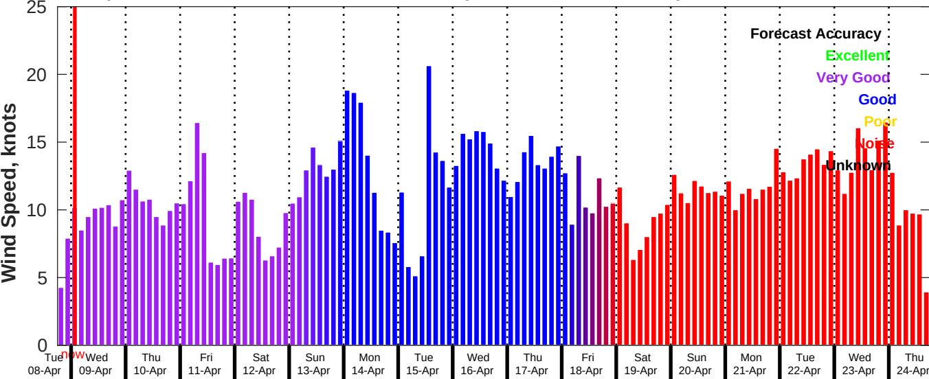
GFS Wind Speed Forecast for NDBC 42035 from 08-Apr-2025 18:00:00 to 24-Apr-2025 18:00:00
