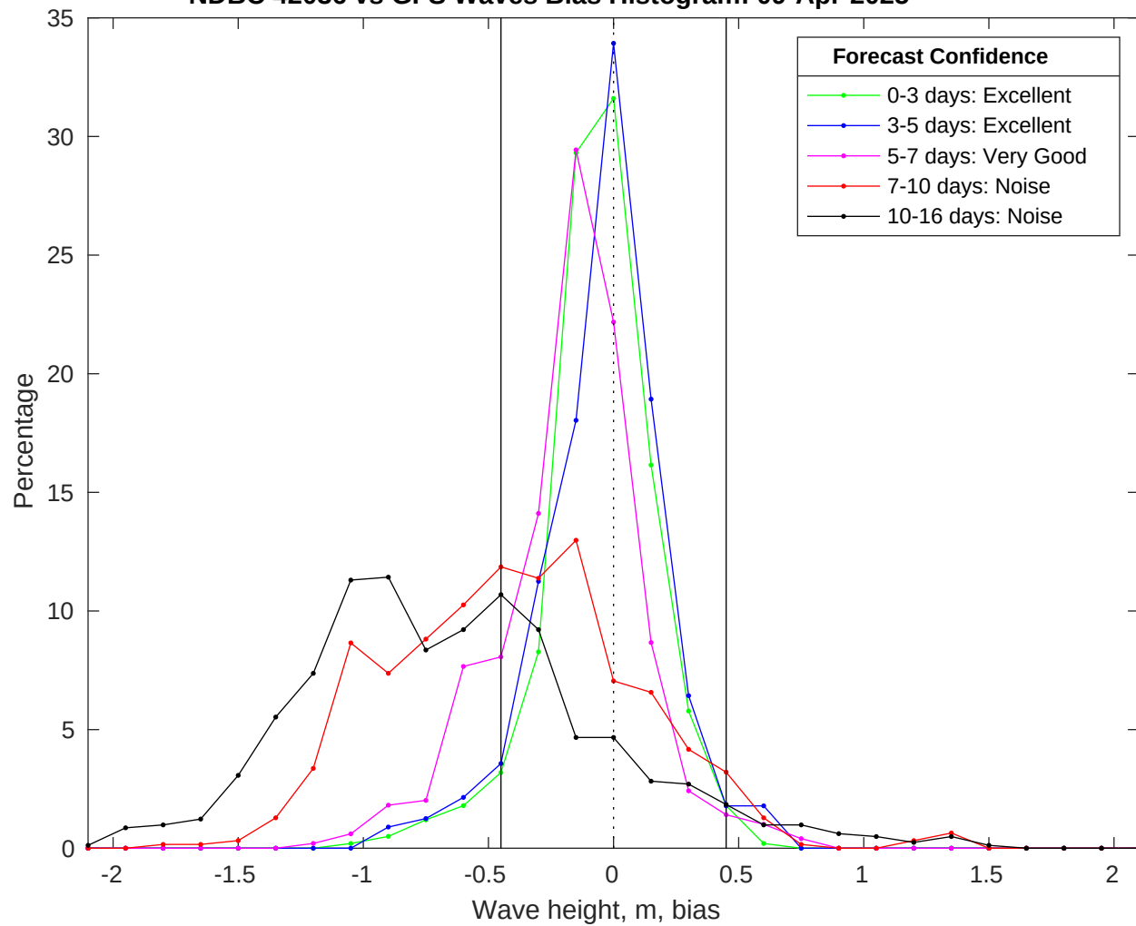
NDBC 42036 vs GFS Waves Bias Histogram: 09-Apr-2025
