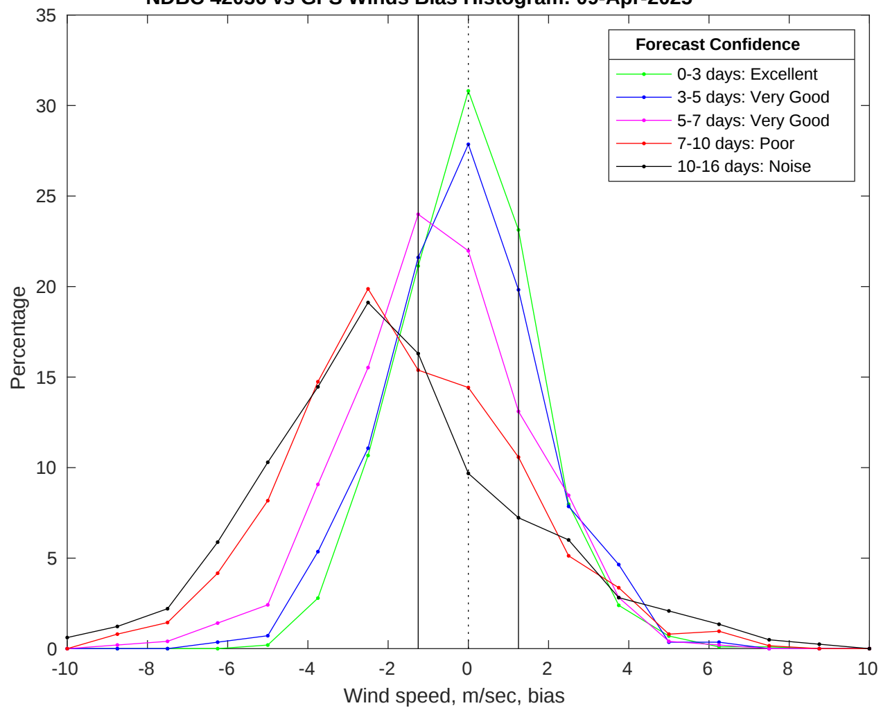
NDBC 42036 vs GFS Winds Bias Histogram: 09-Apr-2025
