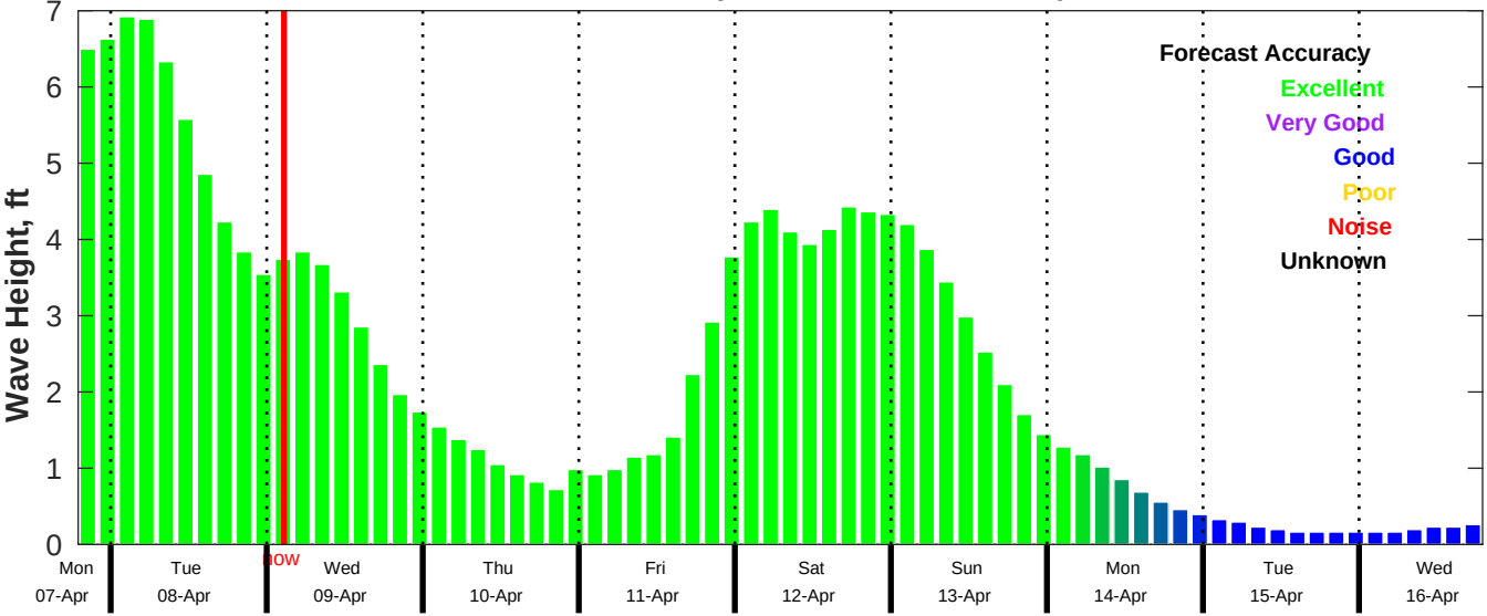
CMEMS Wave Forecast for NDBC 42036 from 07-Apr-2025 19:00:00 to 16-Apr-2025 19:00:00
