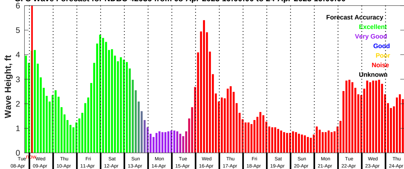
GFS Wave Forecast for NDBC 42036 from 08-Apr-2025 19:00:00 to 24-Apr-2025 19:00:00
