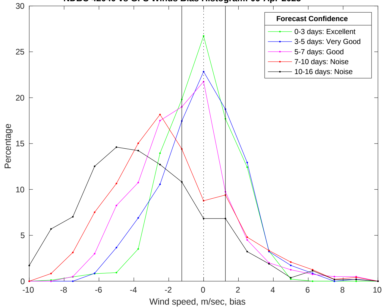
NDBC 42040 vs GFS Winds Bias Histogram: 09-Apr-2025
