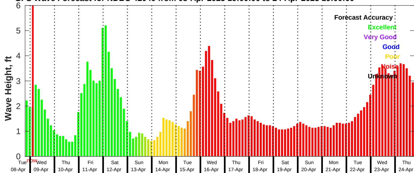
GFS Wave Forecast for NDBC 42040 from 08-Apr-2025 19:00:00 to 24-Apr-2025 19:00:00
