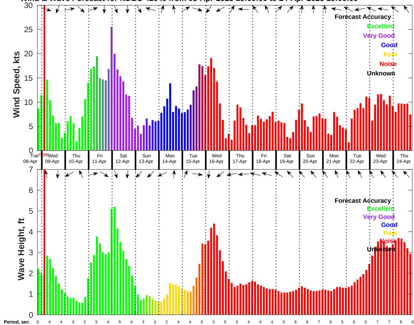
Wind & Wave Forecast for NDBC 42040 from 08-Apr-2025 19:00:00 to 24-Apr-2025 19:00:00
