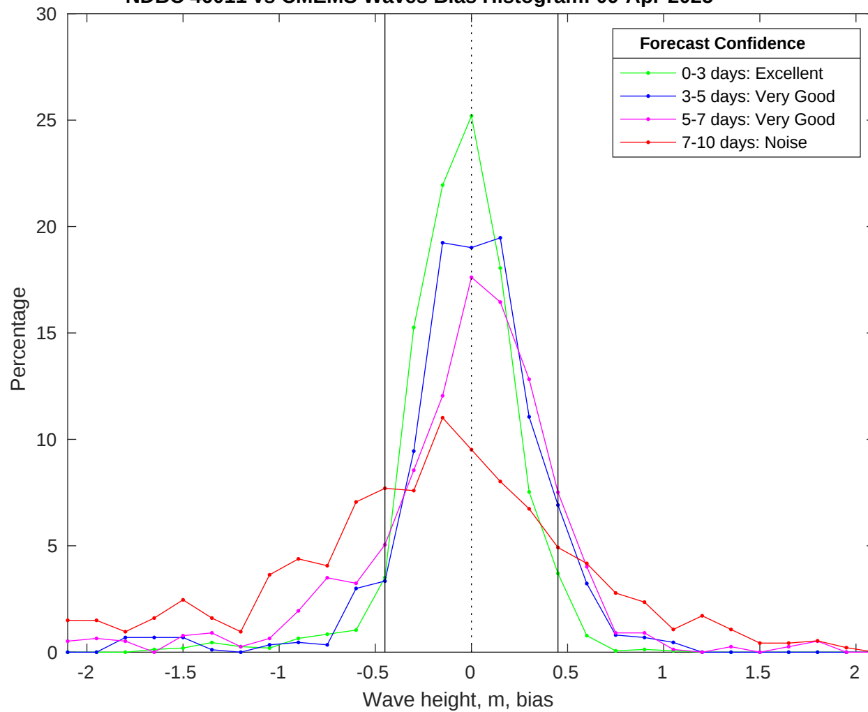
NDBC 46011 vs CMEMS Waves Bias Histogram: 09-Apr-2025
