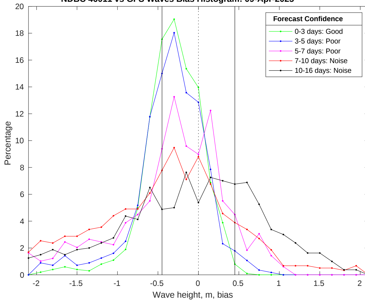
NDBC 46011 vs GFS Waves Bias Histogram: 09-Apr-2025
