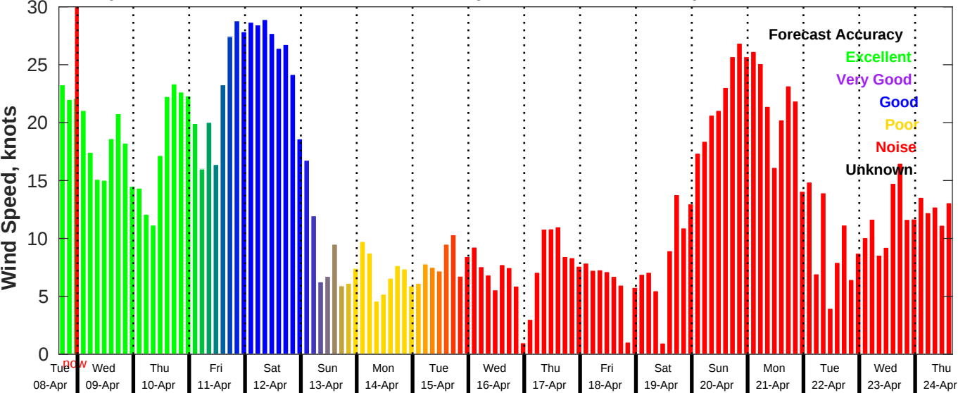
GFS Wind Speed Forecast for NDBC 46011 from 08-Apr-2025 16:00:00 to 24-Apr-2025 16:00:00
