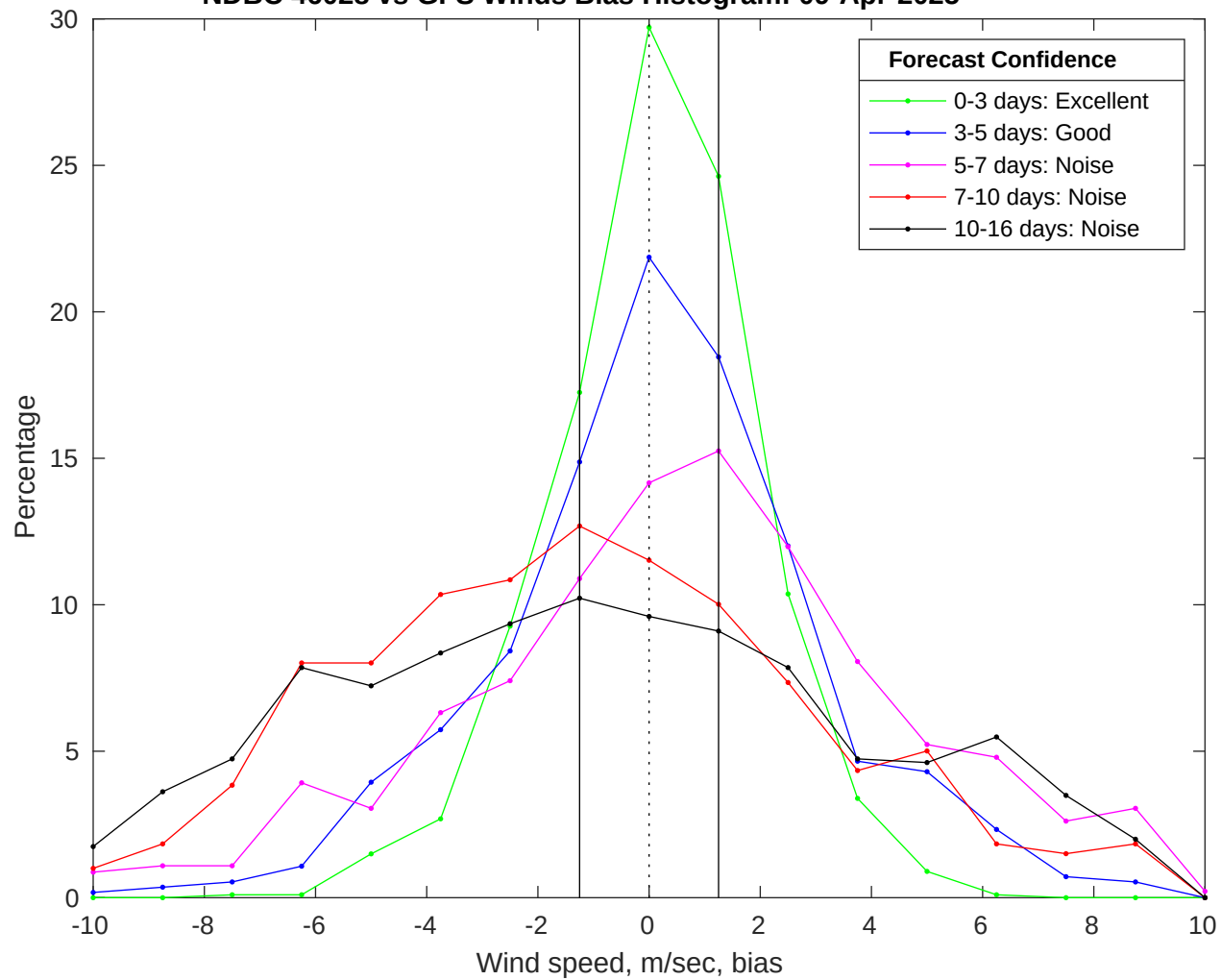
NDBC 46028 vs GFS Winds Bias Histogram: 09-Apr-2025
