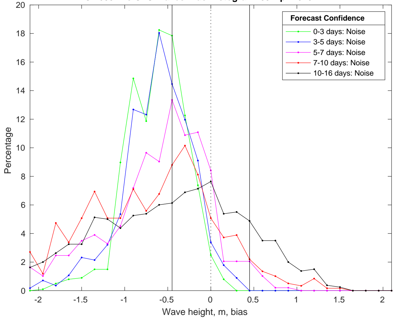
NDBC 46054 vs GFS Waves Bias Histogram: 09-Apr-2025
