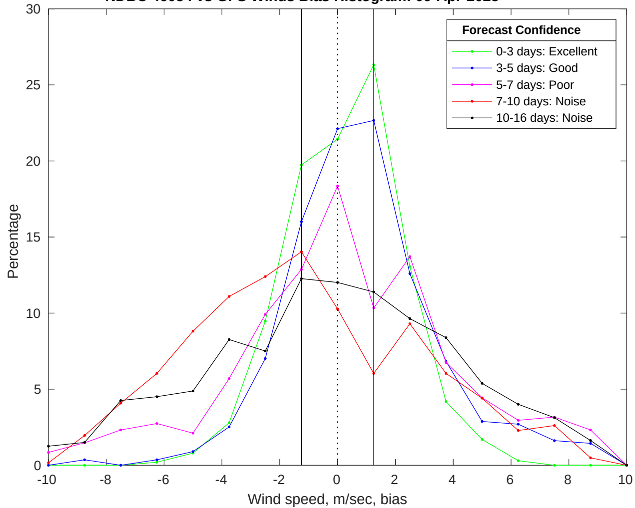
NDBC 46054 vs GFS Winds Bias Histogram: 09-Apr-2025
