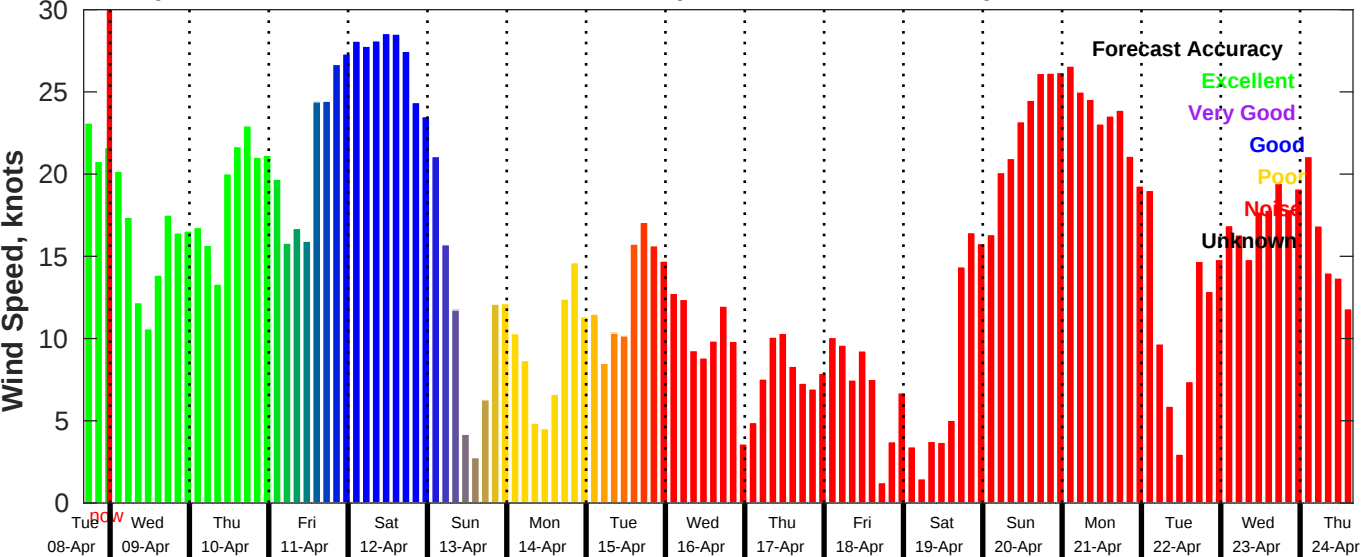
GFS Wind Speed Forecast for NDBC 46054 from 08-Apr-2025 16:00:00 to 24-Apr-2025 16:00:00
