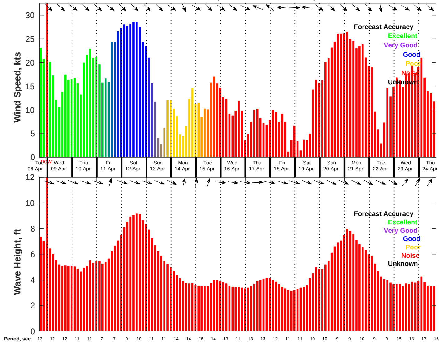
Wind & Wave Forecast for NDBC 46054 from 08-Apr-2025 16:00:00 to 24-Apr-2025 16:00:00
