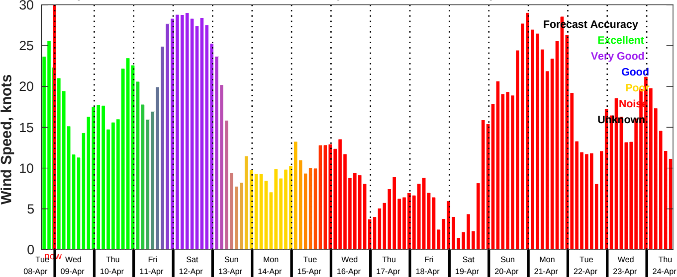
GFS Wind Speed Forecast for NDBC 46069 from 08-Apr-2025 16:00:00 to 24-Apr-2025 16:00:00
