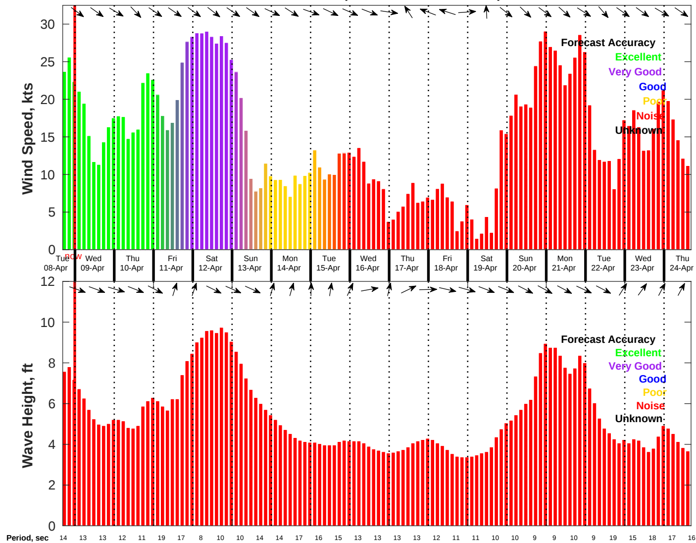
Wind & Wave Forecast for NDBC 46069 from 08-Apr-2025 16:00:00 to 24-Apr-2025 16:00:00
