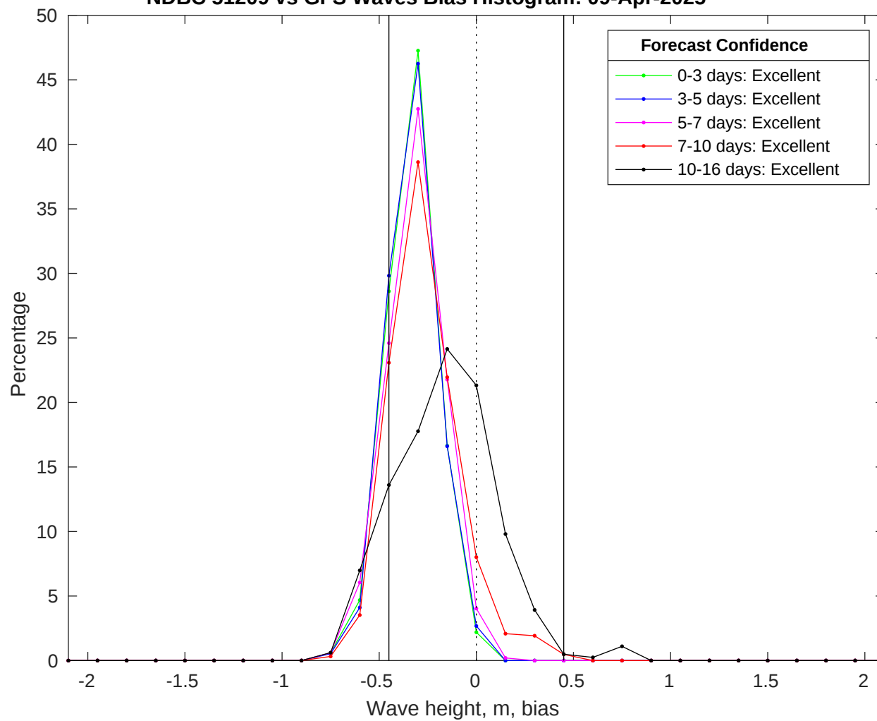
NDBC 51209 vs GFS Waves Bias Histogram: 09-Apr-2025
