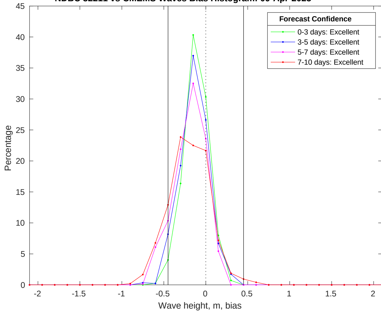
NDBC 52211 vs CMEMS Waves Bias Histogram: 09-Apr-2025
