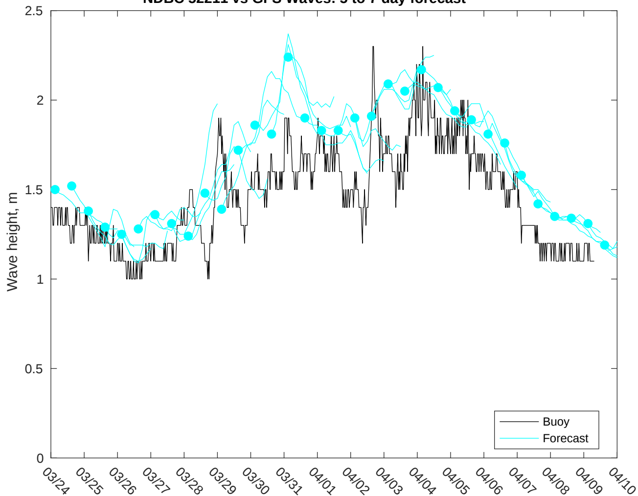
NDBC 52211 vs GFS Waves: 5 to 7 day forecast
