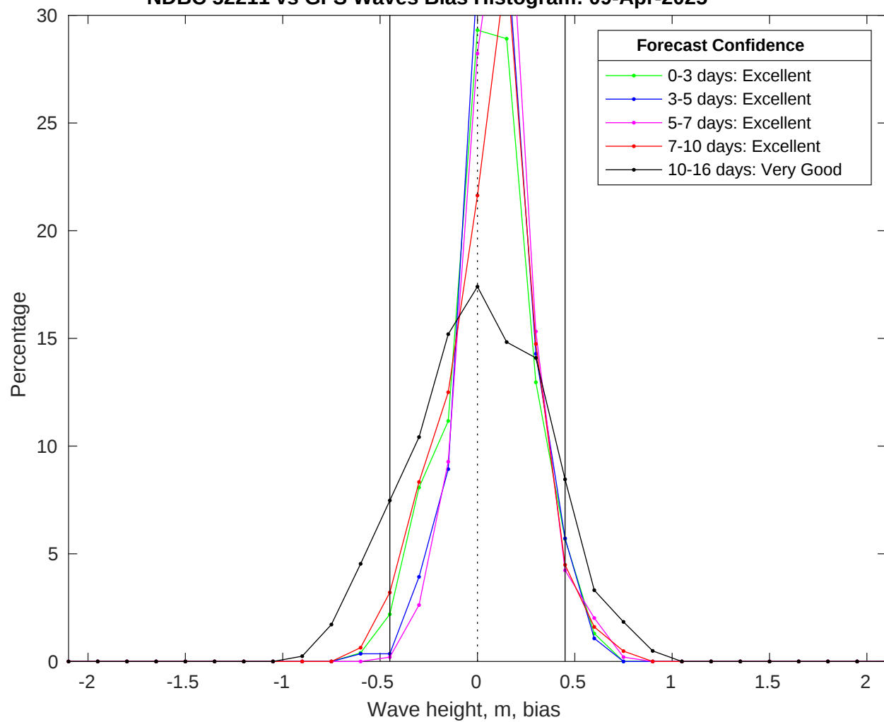
NDBC 52211 vs GFS Waves Bias Histogram: 09-Apr-2025
