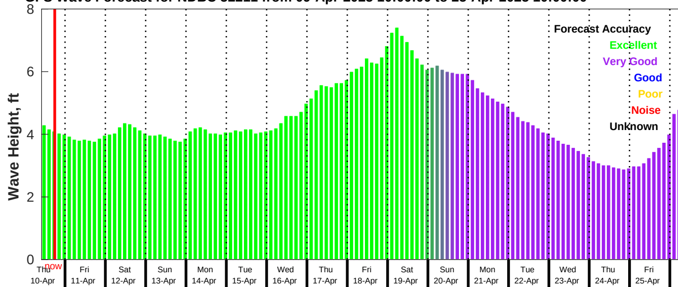
GFS Wave Forecast for NDBC 52211 from 09-Apr-2025 10:00:00 to 25-Apr-2025 10:00:00
